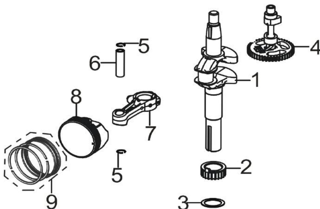
FIG.4 ROD,CRANKSHAFT CONNETING (E04)
