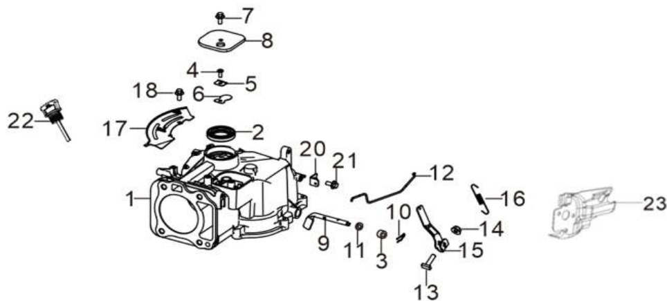
FIG.1 CRANKCASE. / GEAR ASSY, GOVERNOR. (E01)
