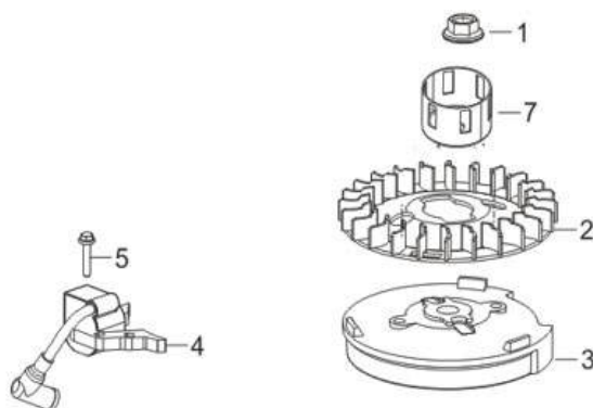
FIG.9 FLYWHEEL / IMPELLER / STARTER PULLEY / IGNITION COIL (E10)
