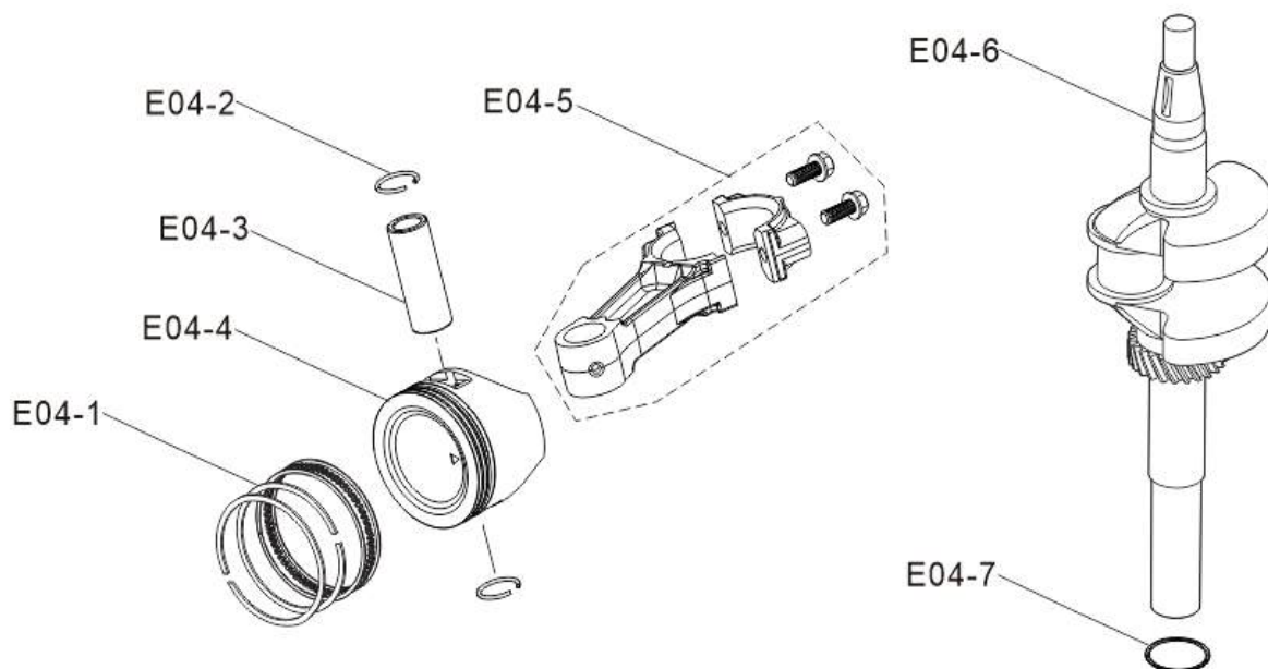
FIG.4 ROD,CRANKSHAFT CONNETING (E04)
