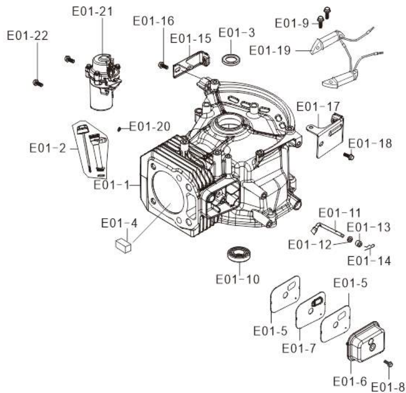
FIG.1 CRANKCASE. / GEAR ASSY, GOVERNOR. (E01)
